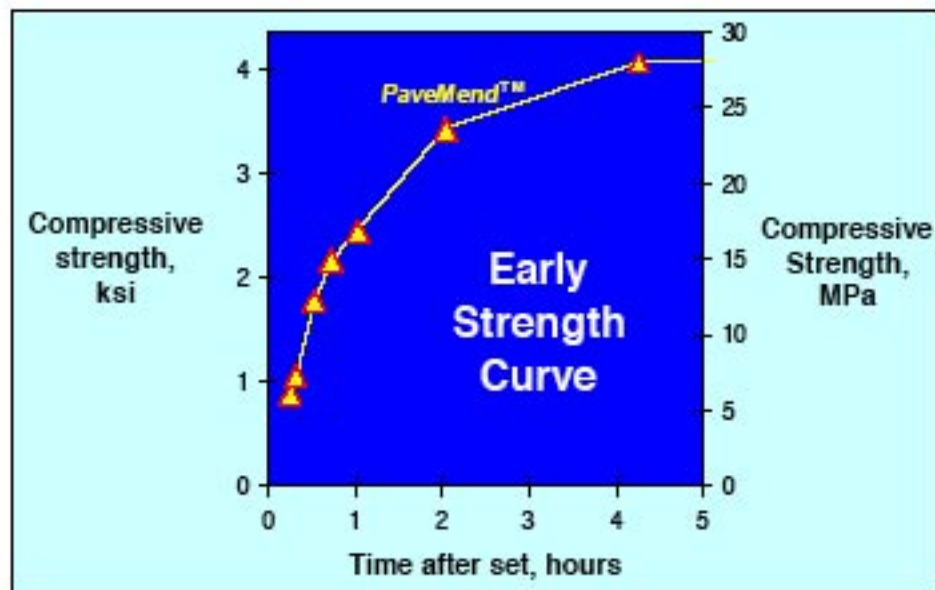
Figure 7. AFRL compressive strength results (expanded time line).
