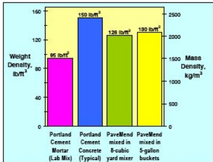
Figure 4. AFRL density test results.
