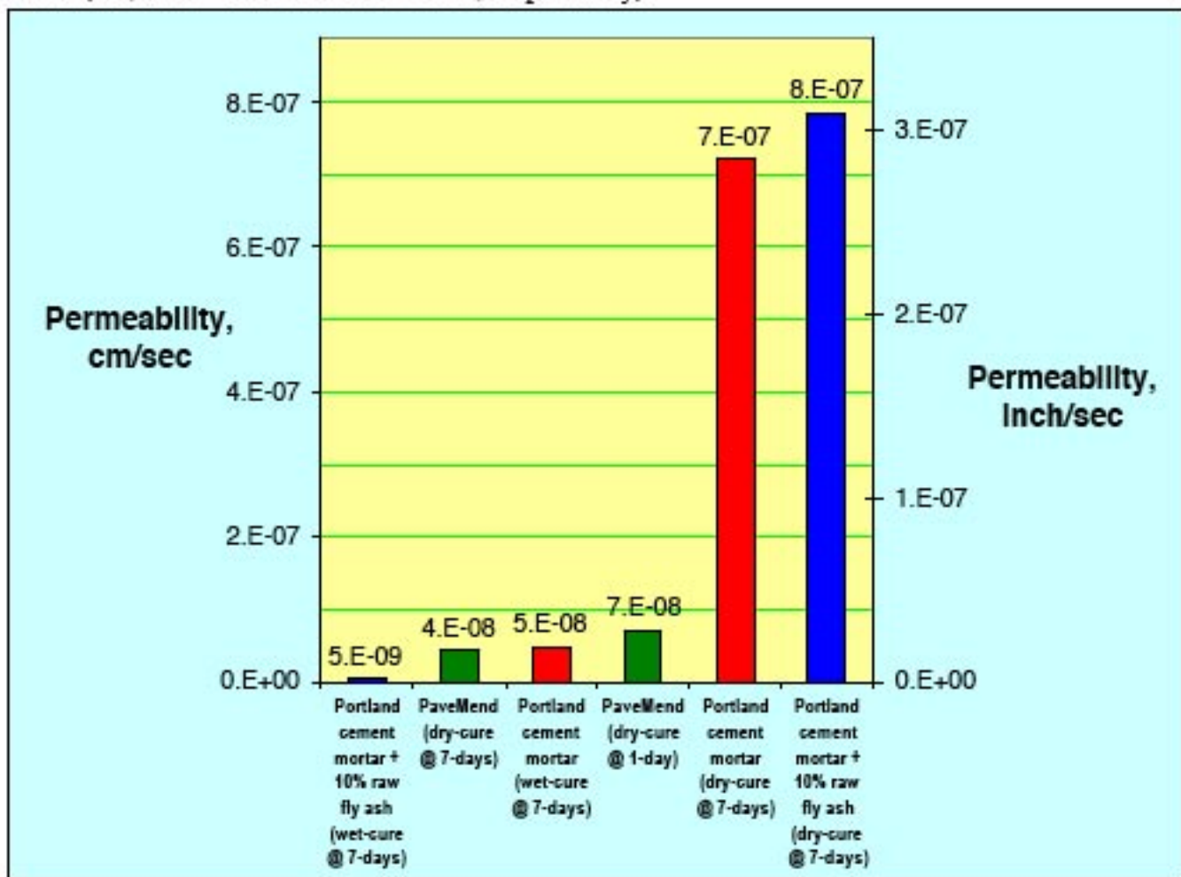
Figure 19. Results of AFRL permeability tests.
