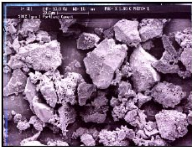
(a) Portland cement particles.
